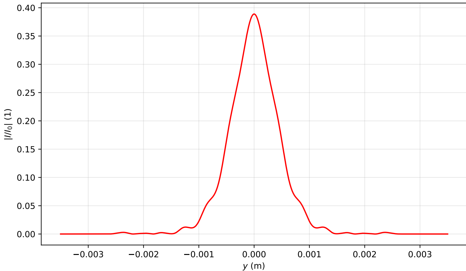
Intensity profile I(x=0, y, z=2.707)/I_0 , P_{in}=1.0P_{cr} , artificial time
